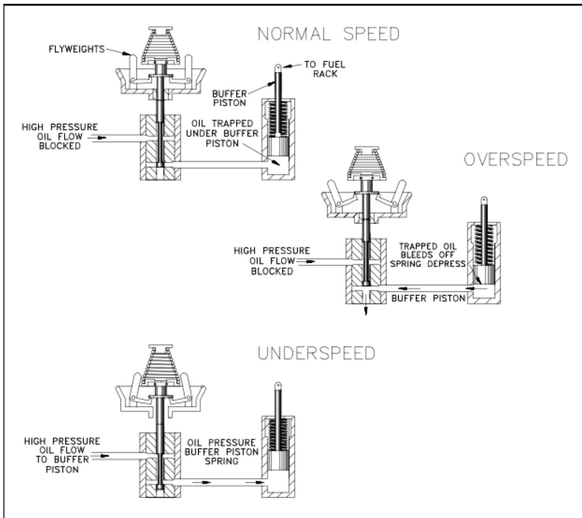
Figure 28 Simplified Mechanical-Hydraulic Governor
