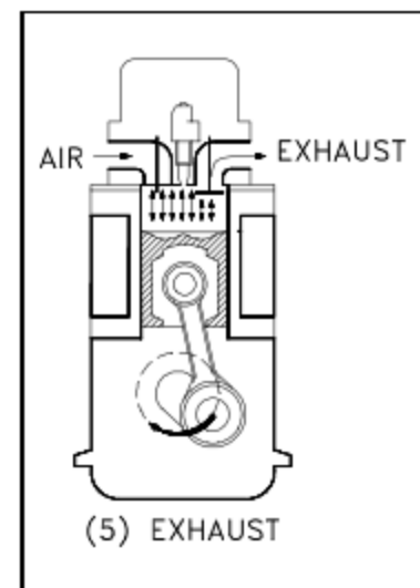
Figure 20 Exhaust
