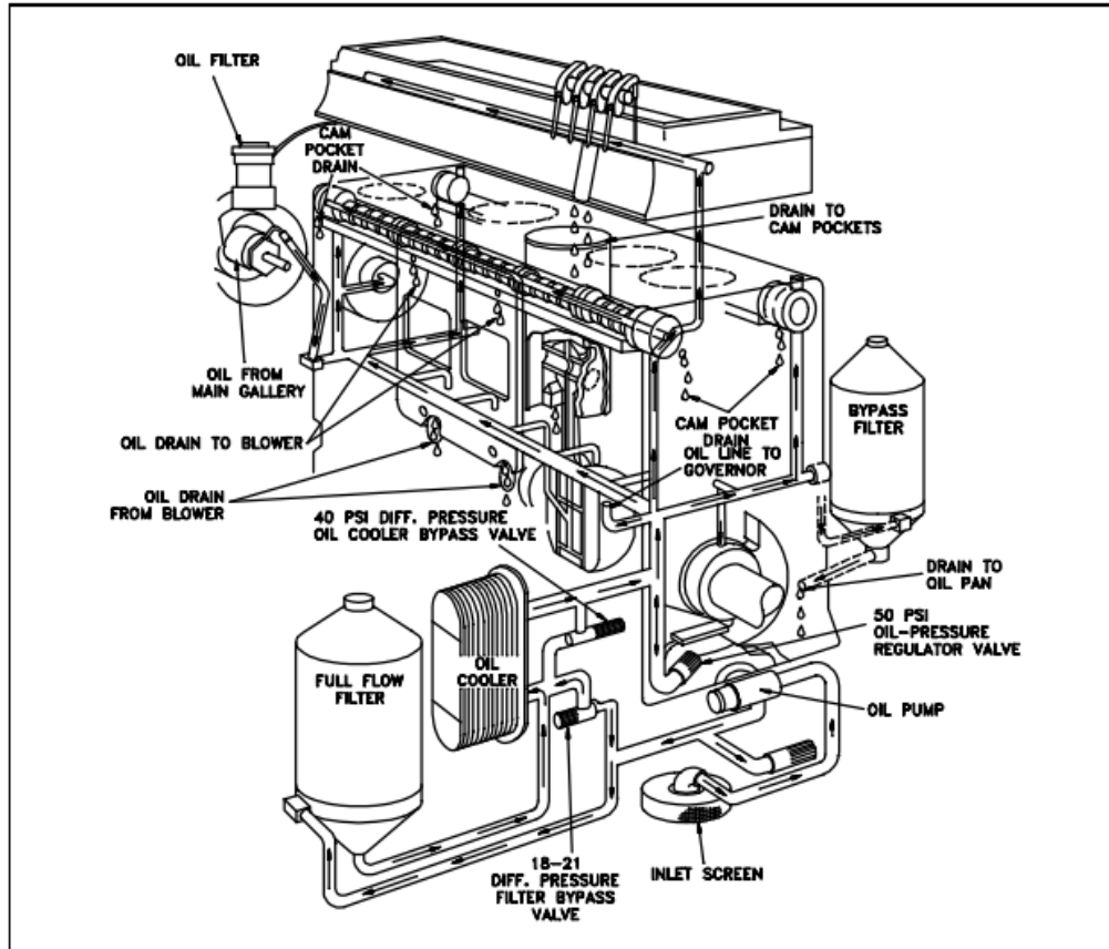
Figure 12 Diesel Engine Internal Lubrication
