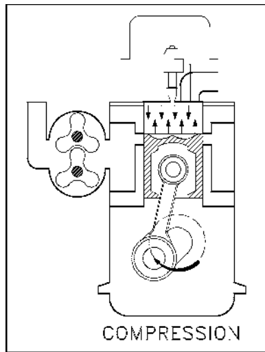
Figure 23 2-Stroke Compression
