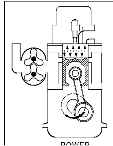
Figure 25 2-Stroke Power
