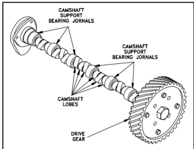
Figure 9 Diesel Engine Camshaft and Drive Gear
