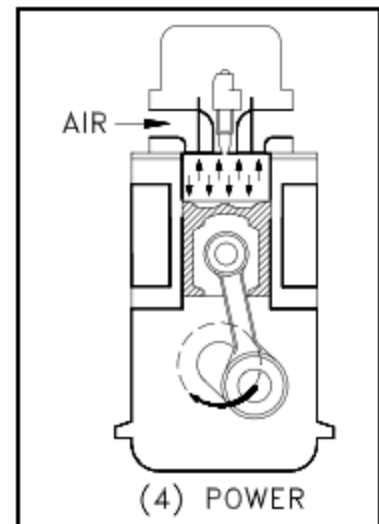
Figure 19 Power
