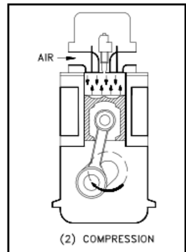
Figure 17 Compression
