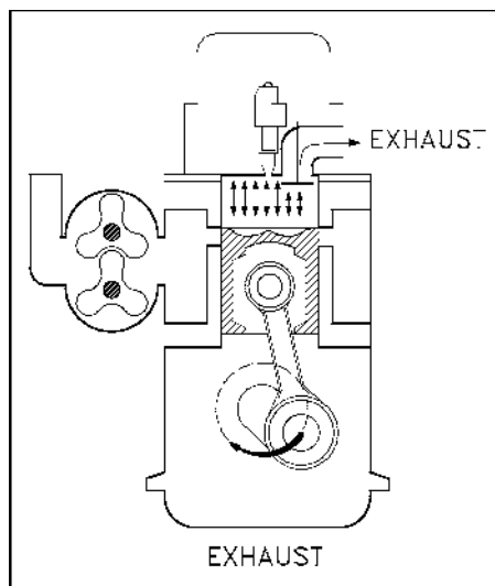
Figure 21 2-Stroke Exhaust
