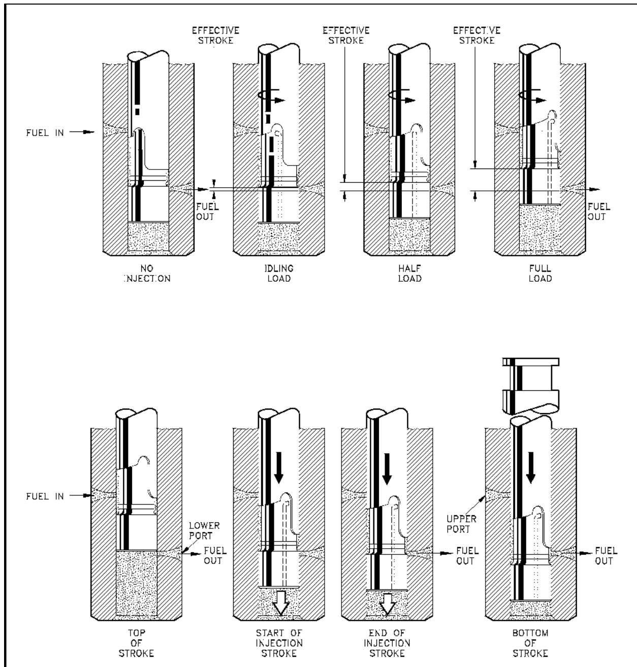
Figure 27 Fuel Injector Plunger
