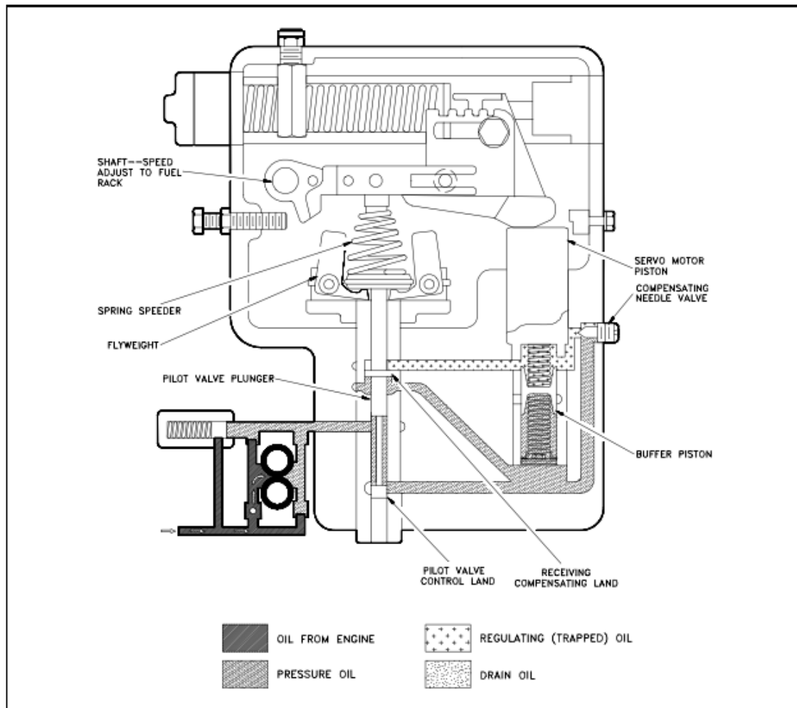
Figure 29 Cutaway of a Woodward Governor
