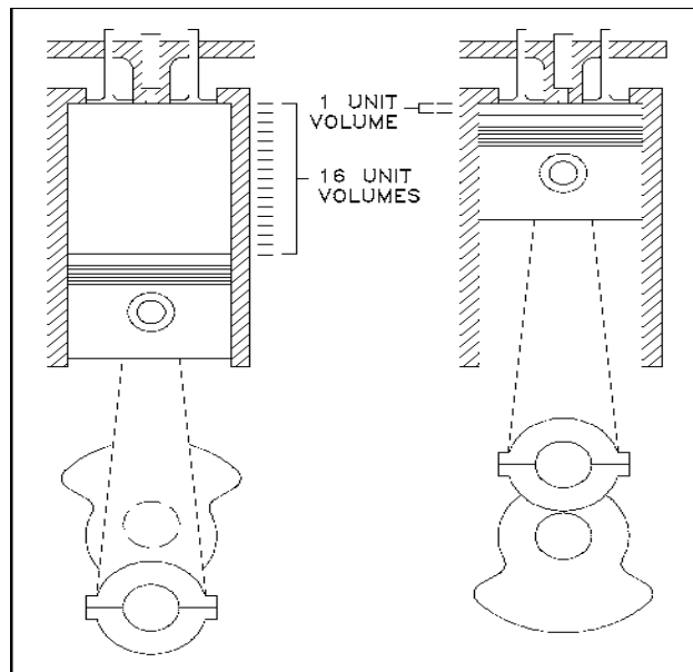
Figure 15 Compression Ratio
